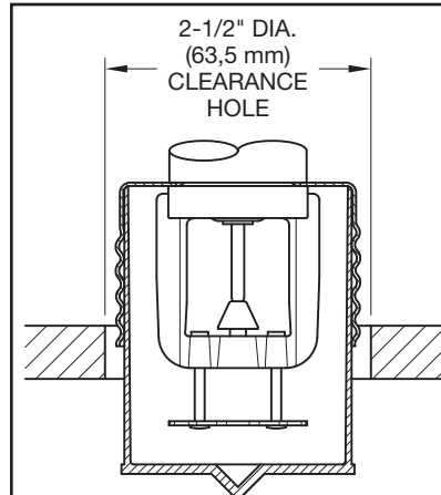
FIGURE 4 DISPOSABLE PROTECTIVE CAP
