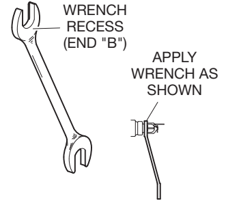
FIGURE 3 W-TYPE 3 SPRINKLER WRENCH
