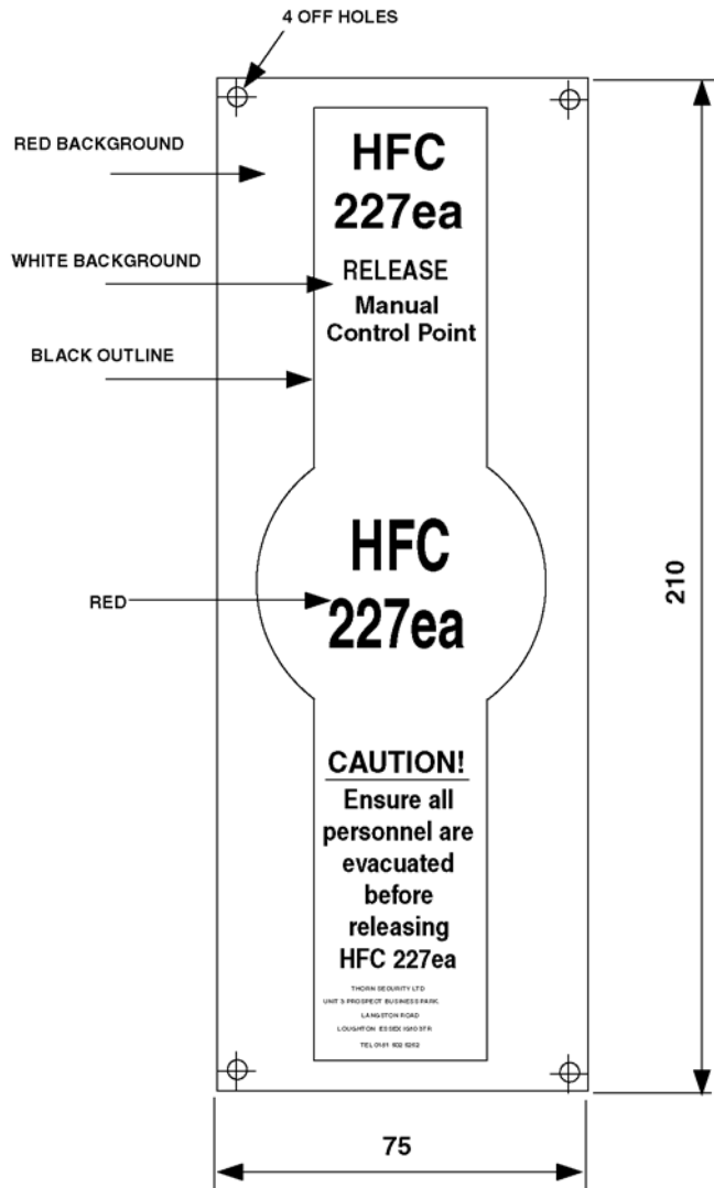
Part No. 314-205-003 Manual Release Caution Plate
