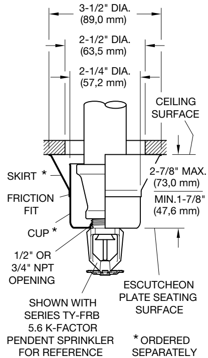
FIGURE 2 STYLE 401 TWO-PIECE DEEP ADJUSTABLE ESCUTCHEON
